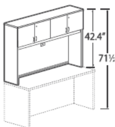
Closed Hutch 72"W x 42" H
